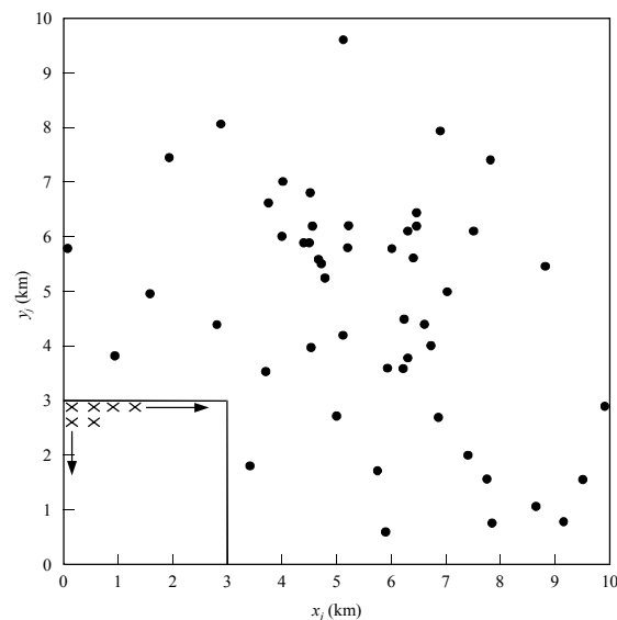
Figure 3: Sampling locations using algorithm in Rec. 1599
