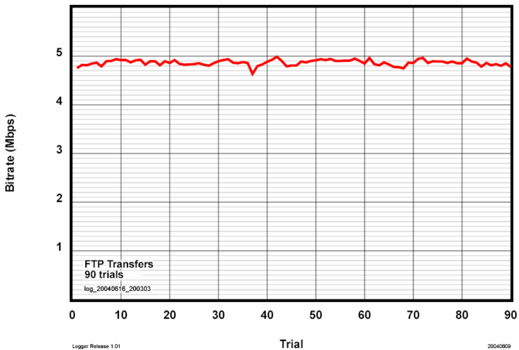
Figure 35: Measured throughput in 802.11b
