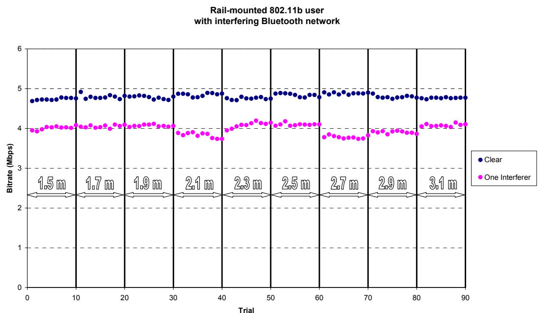
Figure 42: Effect of adding interfering Bluetooth network
