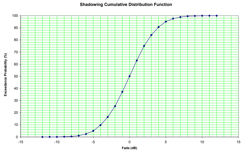
Figure 17: Shadowing Cumulative Distribution Function (dB)
