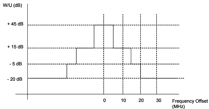
Figure D2: W/U for analogue FM RX with CW interference
