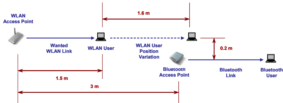
Figure 34: Experimental configuration
