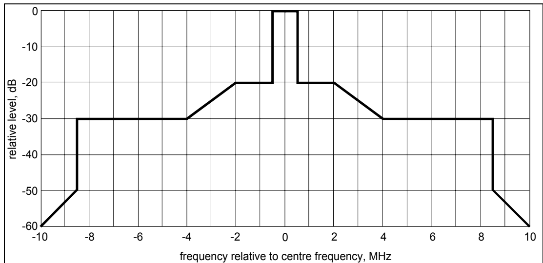
Figure D1: Representative spectrum mask for analogue ENG/OB video links
