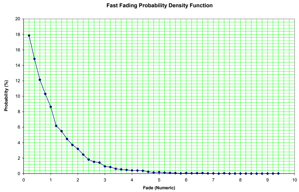
Figure 14: Fast-fading Probability Density Function (Numeric)
