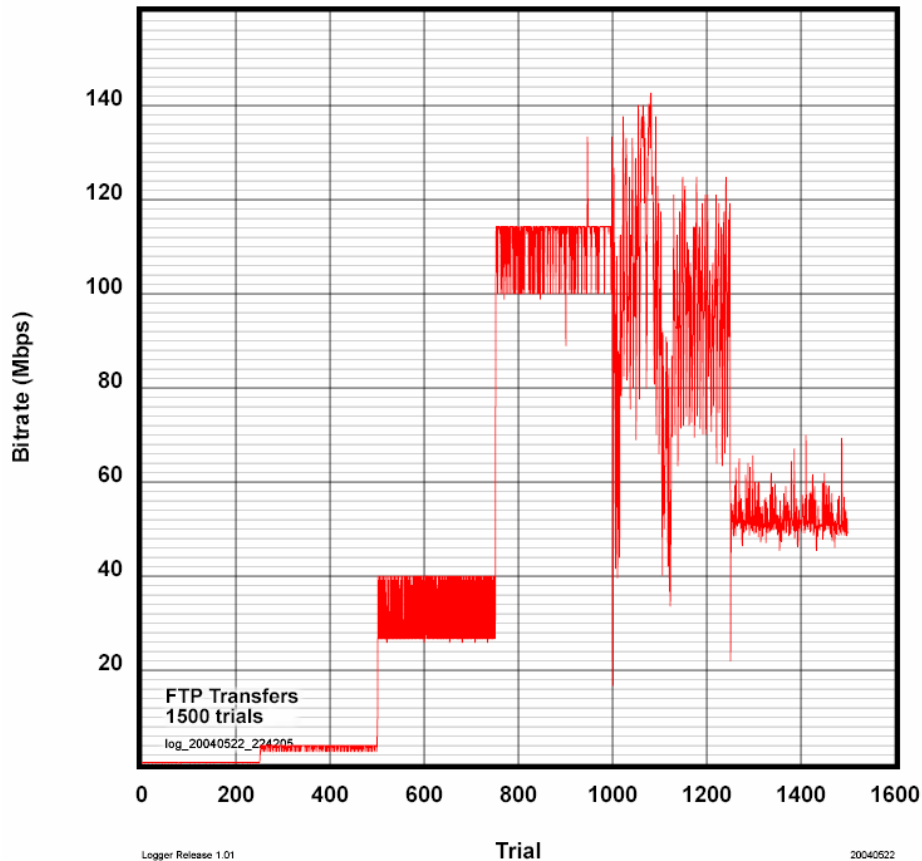
Figure 37: FTP performance and file size
