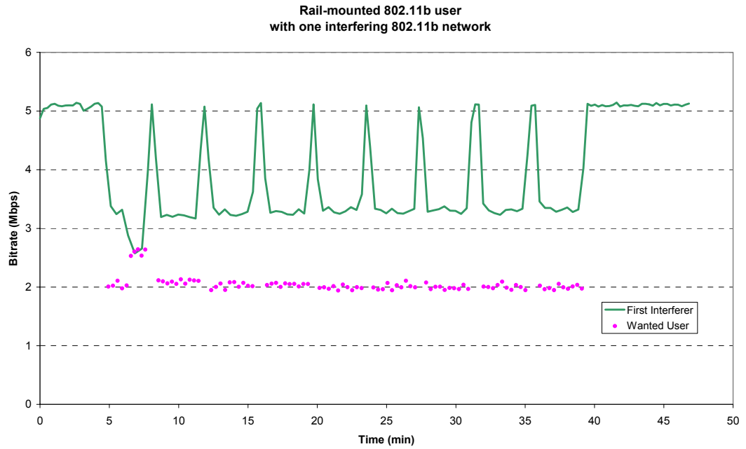
Figure 40: Throughput variation with time (one 802.11b interferer)
