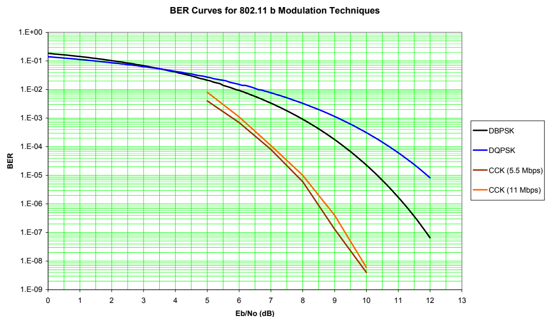
Figure 20: BER performance for 802.11b modulation techniques
