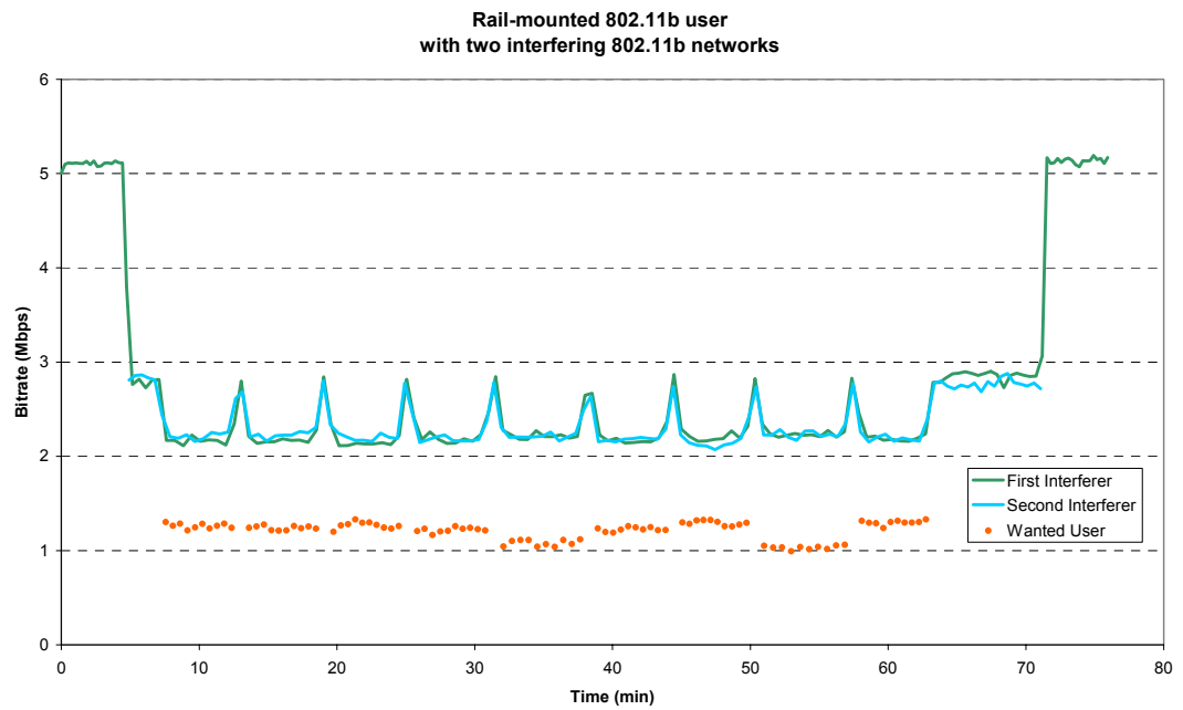
Figure 41: Throughput variation with time (two 802.11b interferers)
