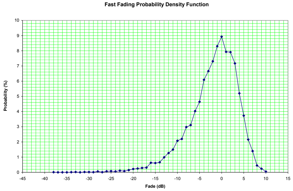
Figure 12: Fast-fading Probability Density Function (dB)
