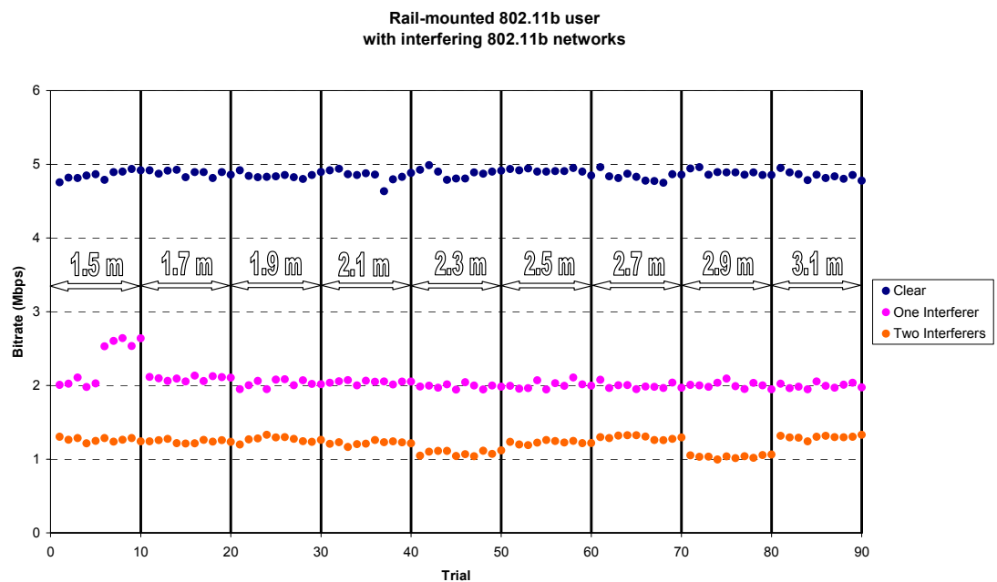
Figure 39: Effect of adding interfering 802.11b networks
