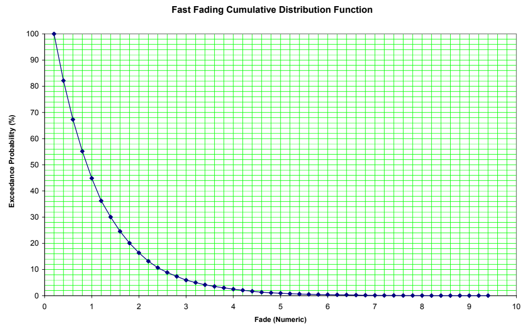
Figure 15: Fast-fading Cumulative Distribution Function (Numeric)
