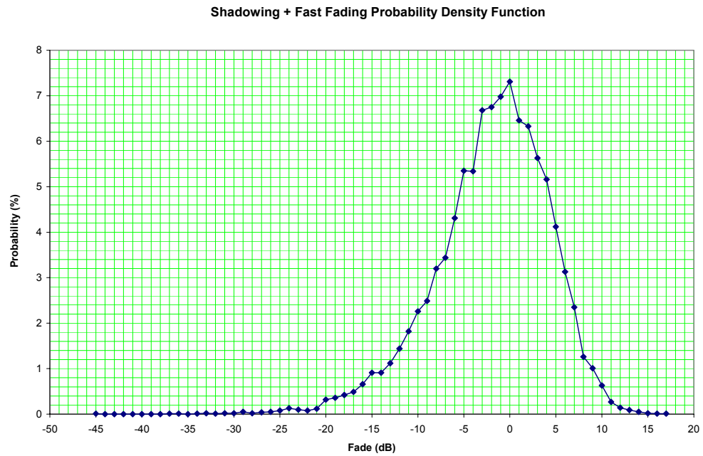
Figure 18: Fast-fading and shadowing Probability Density Function (dB)
