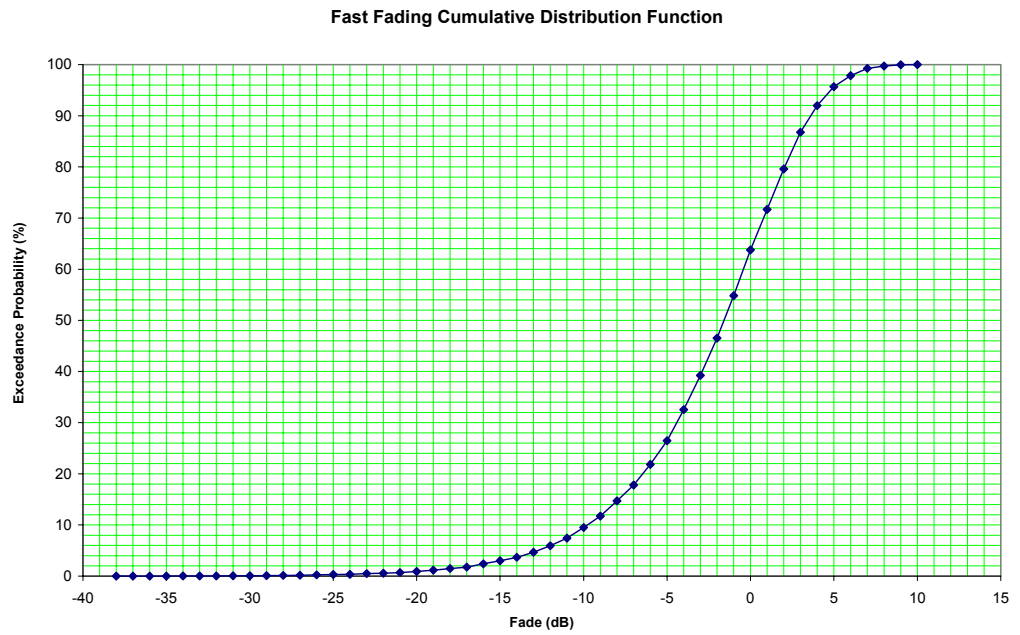
Figure 13: Fast-fading Cumulative Distribution Function (dB)
