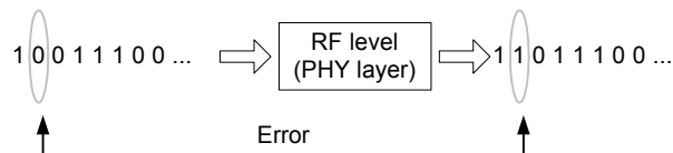
Figure 2: PHY layer bit error model
