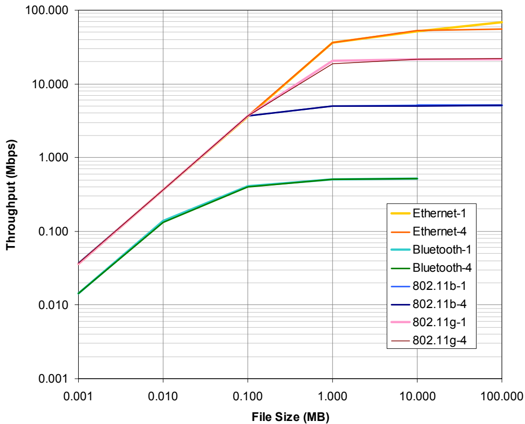
Figure 38: FTP throughput
