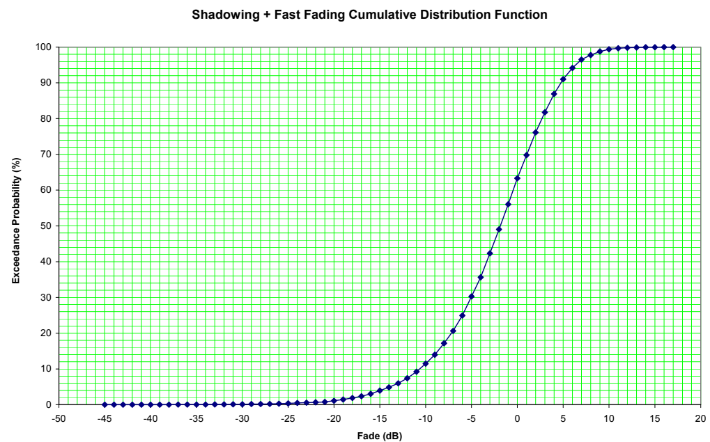
Figure 19: Fast-fading and shadowing Cumulative Distribution Function (dB)
