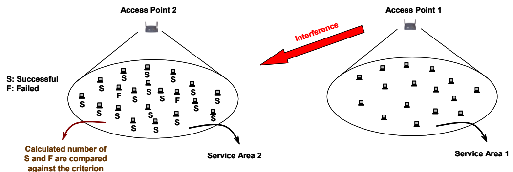
Figure 22: Location dependency
