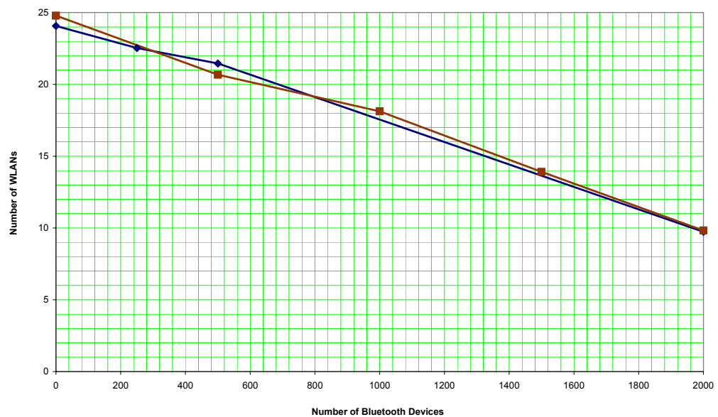
Figure 26: Number of WLANs vs number of Bluetooth devices
