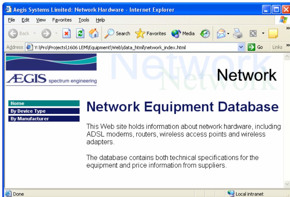
Figure 36: Equipment database
