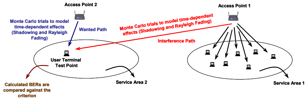
Figure 21: Example scenario
