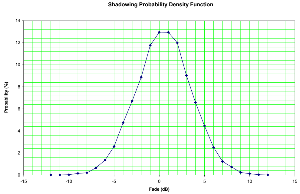
Figure 16: Shadowing Probability Density Function (dB)
