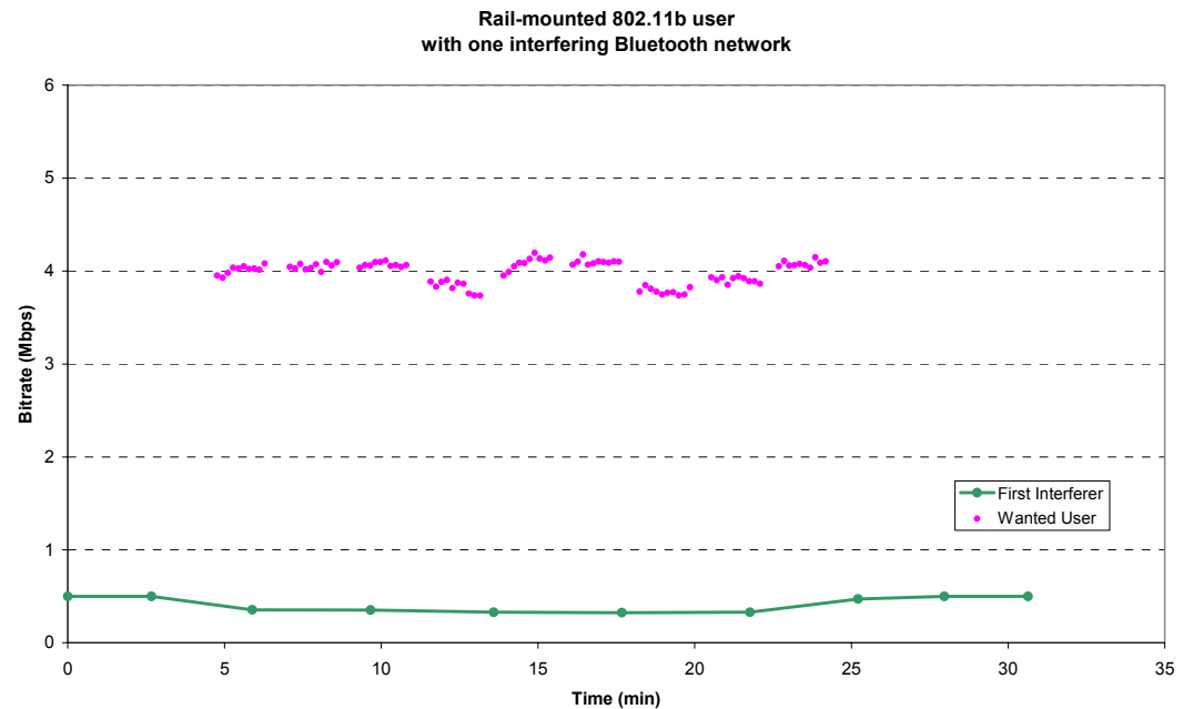
Figure 43: Throughput variation with time (one Bluetooth interferer)
