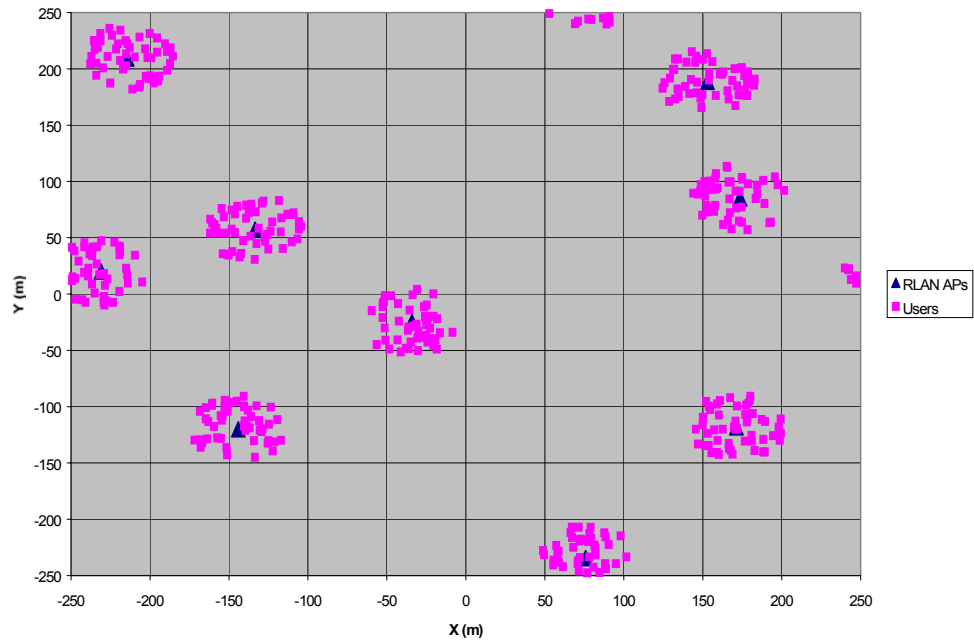
Figure 24: Typical distribution of WLAN access points and users
