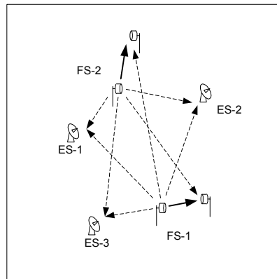
Figure 7: Interference paths for example FS-ES deployment
