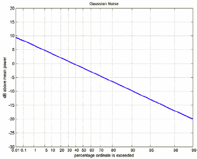
Figure 4.7 : APD in 36 MHz Bandwidth of Gaussian Noise (Generated by a Noise Diode)
