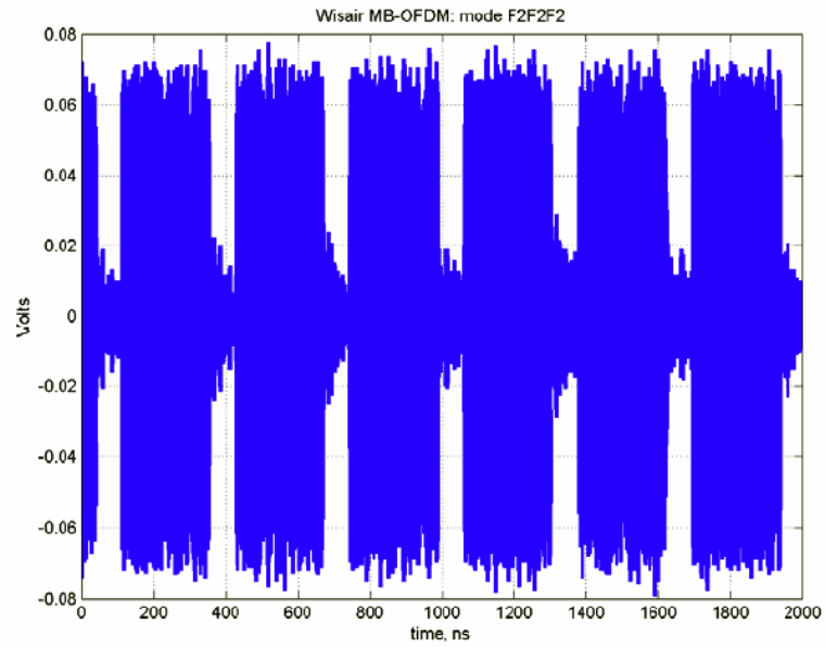
Figure 4.14 : MB-OFDM Emission in A Non-Hopping Mode in the Time Domain (Taken from an ITS NTIA document titled 'Task 1 Report of A Study to Define Metrics that Determine the Interference Potential of Various UWB Waveforms')
