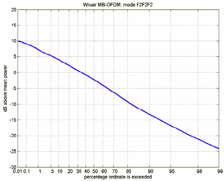
Figure 4.12 : APD in 36 MHz Bandwidth of MB-OFDM Emission in A Non-Hopping Mode (TX Designed to Hop In The First Band Group) (Taken from an ITS NTIA document titled ‘Task 1 Report of A Study to Define Metrics that Determine the Interference Potential of Various UWB Waveforms’)
