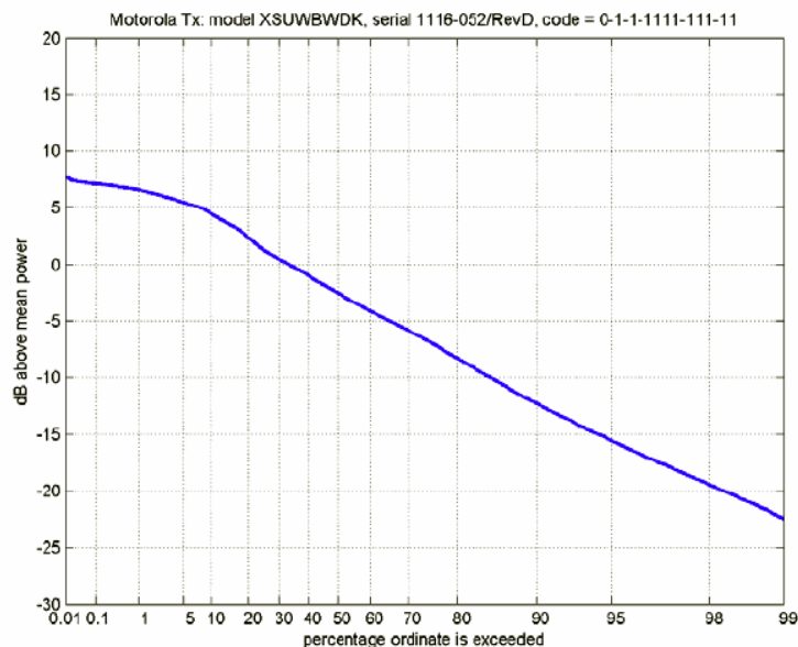
Figure 4.4 : APD in 36 MHz Bandwidth of DS-UWB Emission (TX Designed to Operate In The Lower Band (3.1–4.85 GHz) with BPSK Modulation and Code Length 12) (Taken from an ITS NTIA document titled ‘Task 1 Report of A Study to Define Metrics that Determine the Interference Potential of Various UWB Waveforms’)
