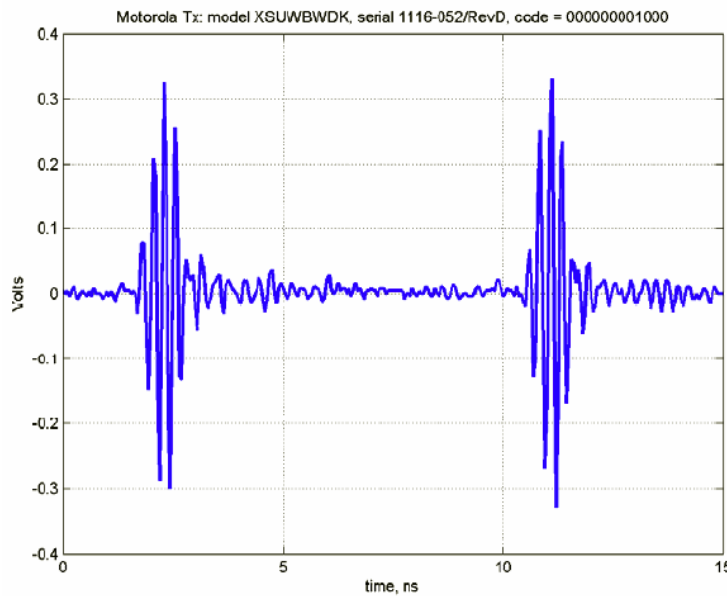
Figure 4.6 : DS-UWB Emission in the Time Domain (Taken from an ITS NTIA document titled ‘Task 1 Report of A Study to Define Metrics that Determine the Interference Potential of Various UWB Waveforms’)
