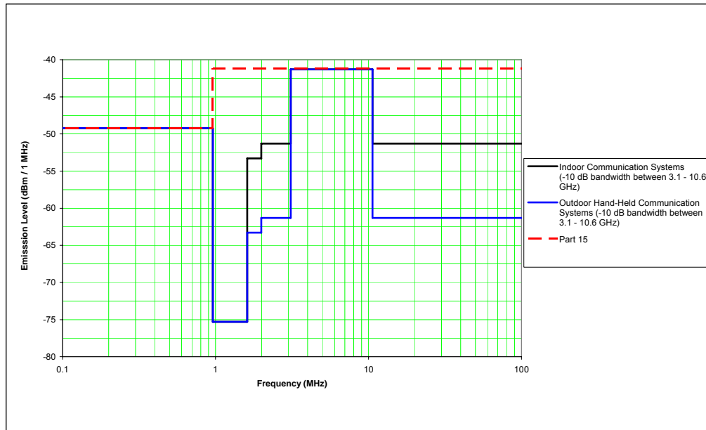
Figure 2.1: FCC mask for UWB devices
