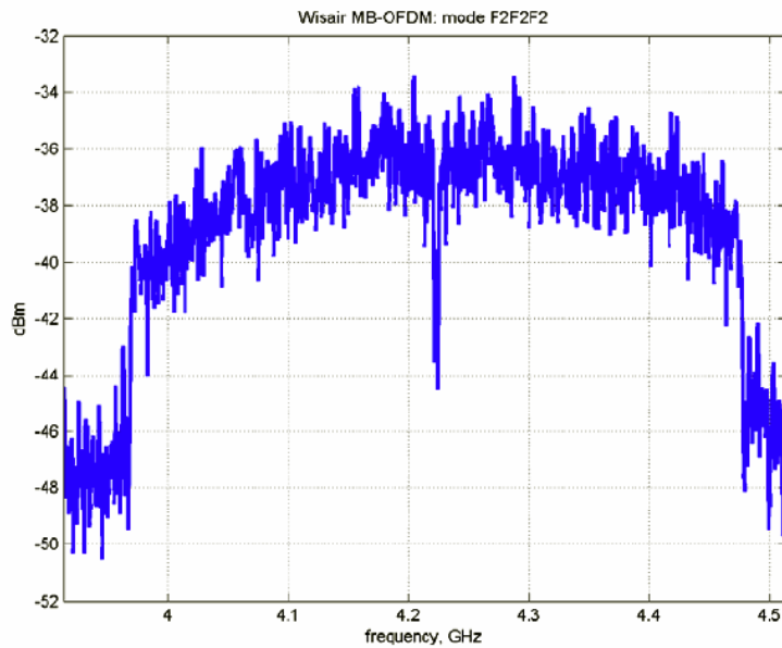
Figure 4.13 : Spectrum Plot of MB-OFDM Emission in A Non-Hopping Mode (Taken from an ITS NTIA document titled ‘Task 1 Report of A Study to Define Metrics that Determine the Interference Potential of Various UWB Waveforms’)
