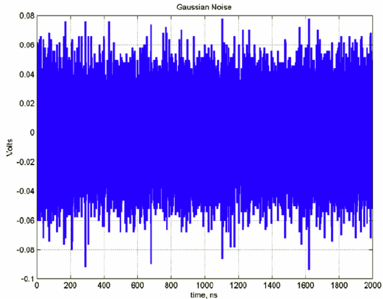
Figure 4.9 : Gaussian Noise Emission in the Time Domain (Taken from an ITS NTIA document titled ‘Task 1 Report of A Study to Define Metrics that Determine the Interference Potential of Various UWB Waveforms’)
