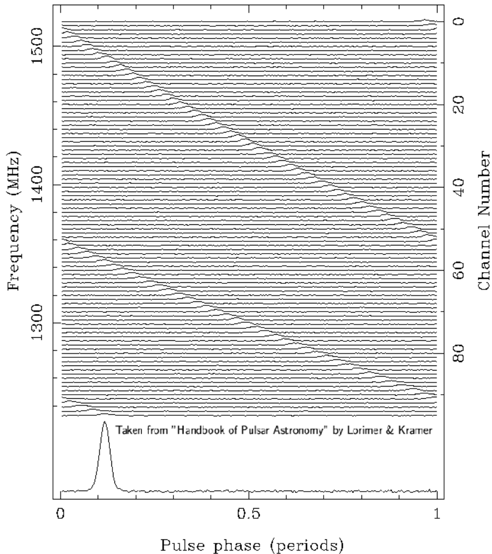
Figure 3.3: showing pulse dispersion
