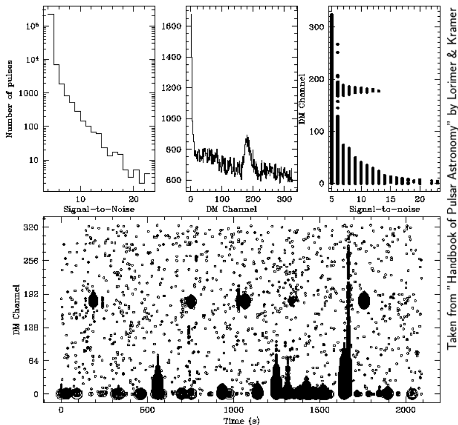
Figure 3.4: Showing pulsar, with zero-dispersion interference
