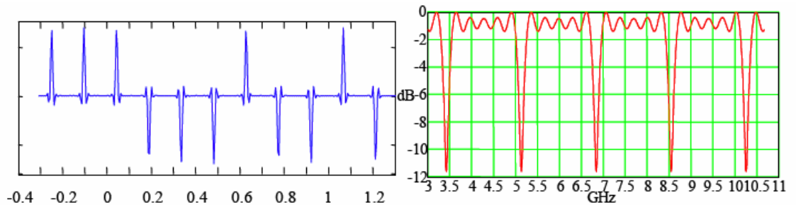
Figure 4.2 : Example Code Sequence in Time and Frequency Domain (Taken from a document provided by Freescale Semiconductor titled ‘Key Attributes of DS-UWB & Answers to Frequently Asked Questions’, 31.May.2005)
