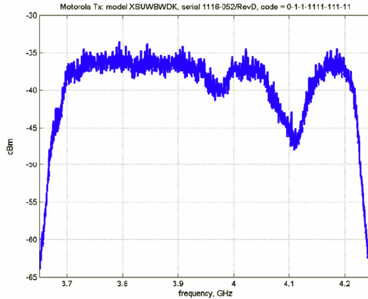
Figure 4.5 : Spectrum Plot of DS-UWB Emission (Taken from an ITS NTIA document titled ‘Task 1 Report of A Study to Define Metrics that Determine the Interference Potential of Various UWB Waveforms’)
