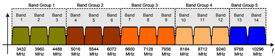
Figure 4.10: MB-OFDM Bands
