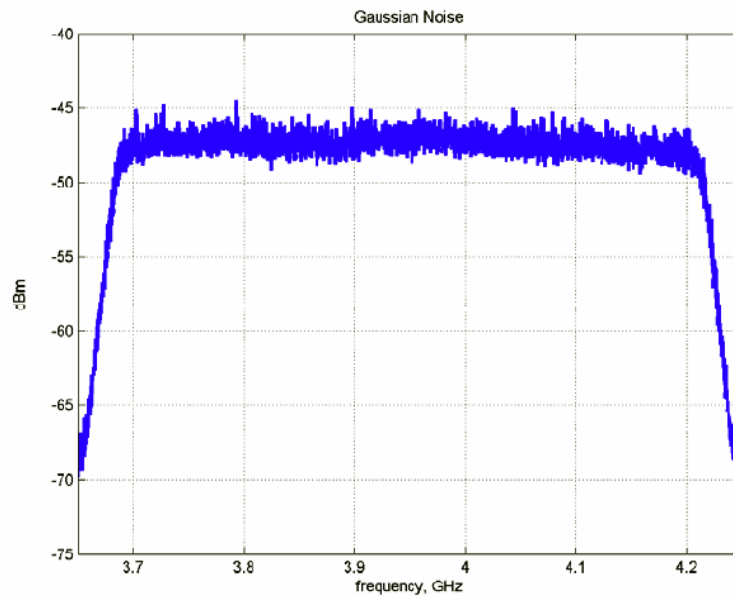
Figure 4.8 : Spectrum Plot of Gaussian Noise
