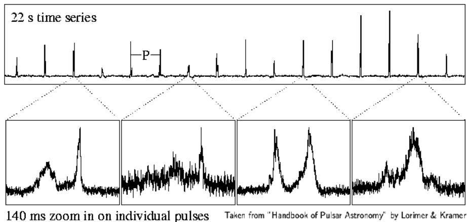
Figure 3.1: Pulse series from typical pulsar (Arecibo telescope)
