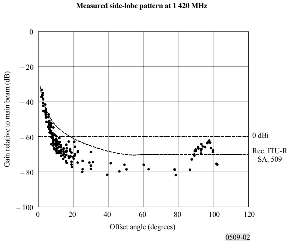
Figure 3.6: Lovell telescope sidelobe measurements
