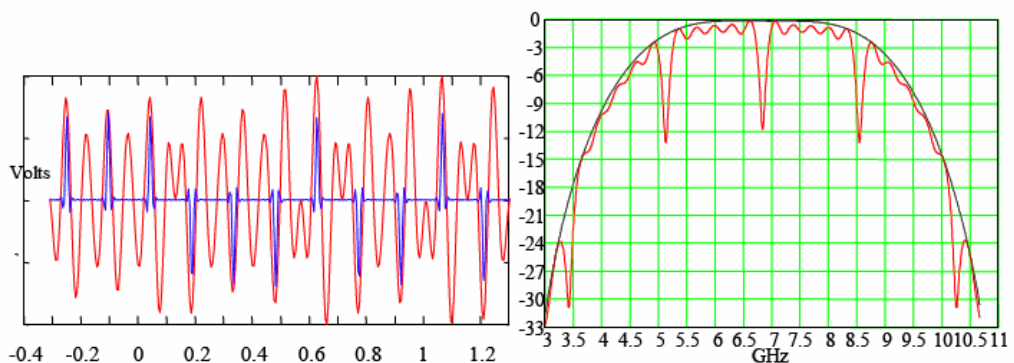
Figure 4.3 : Example DS-UWB signal in Time and Frequency Domain (Taken from a document provided by Freescale Semiconductor titled ‘Key Attributes of DS-UWB & Answers to Frequently Asked Questions’, 31.May.2005)
