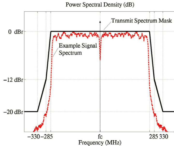
Figure 4.11: MB-OFDM Transmit Power Spectral Mask
