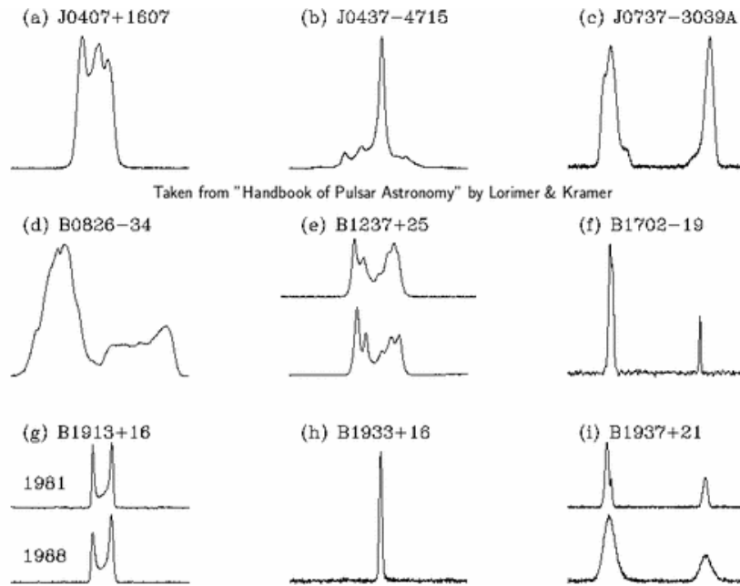
Figure 3.2: Showing the variety of pulse profiles
