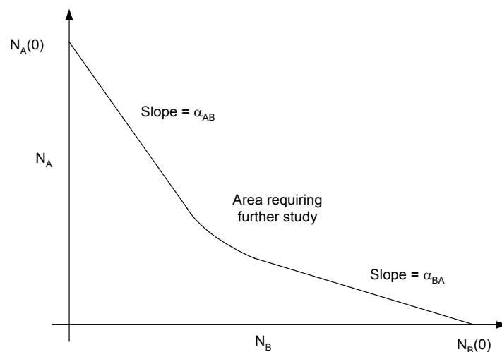
Figure 3.4 The mutual interference between Systems of type A and B
