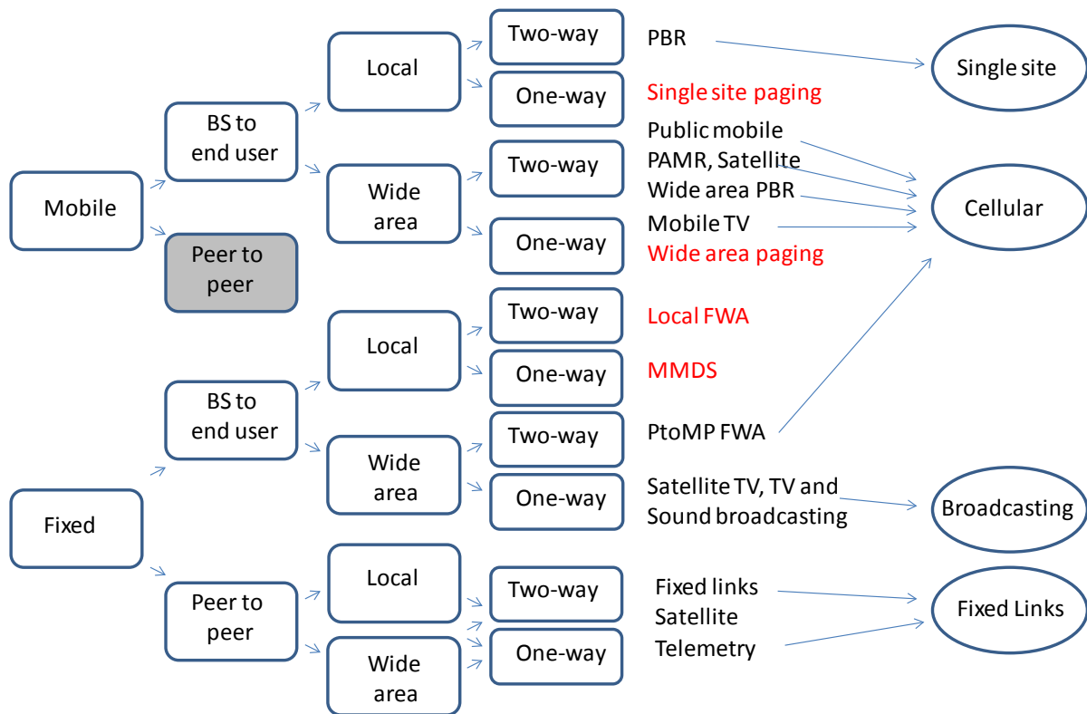
Figure 3-1: Applications and reference networks
