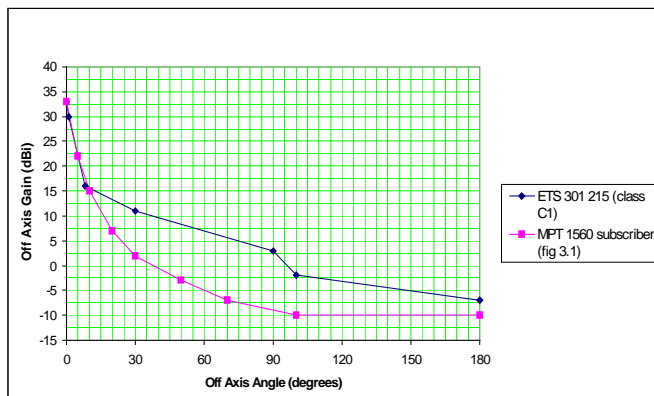
Directional, 33 dBi
