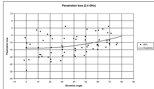
Figure 3: Elevation dependence 2.4 GHz (all locations)
