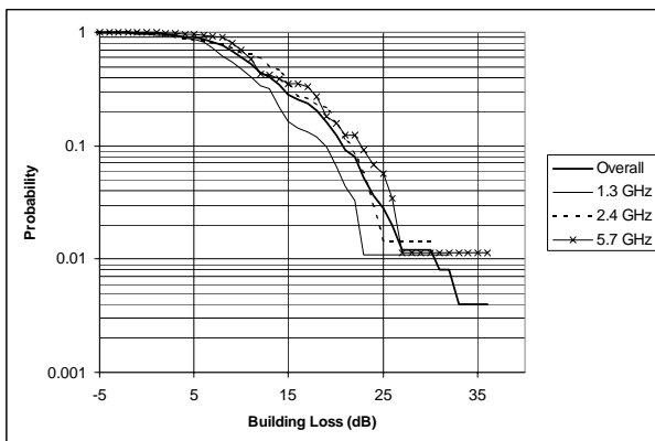
Figure 2: Overall statistics of building penetration loss
