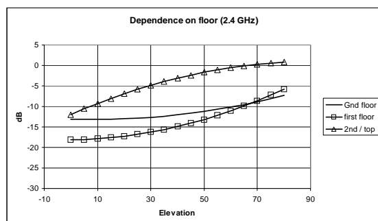
Figure 5: Loss dependence on building floor (2.4 GHz)
