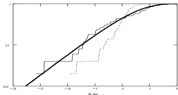
Figure 6: Small-scale fading – Comparison of 'Test' (solid) and 'Reference' (dotted) measurements with Rayleigh statistics
